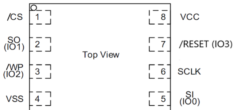
Figure 1c. Pad Configuration
