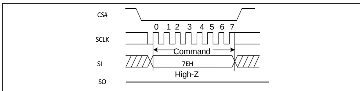
Figure 46a Global Block/Sector Lock Sequence Diagram (SPI)
