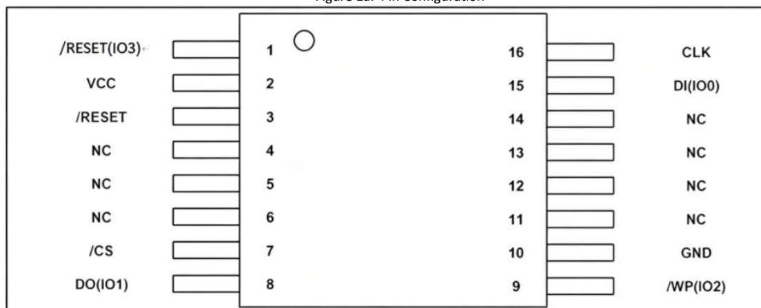
Figure 1a. Pin Configuration
