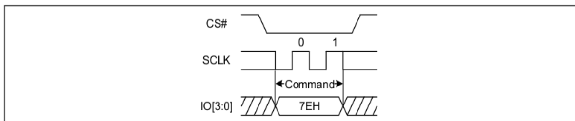
Figure 46b Global Block/Sector Lock Sequence Diagram (QPI)
